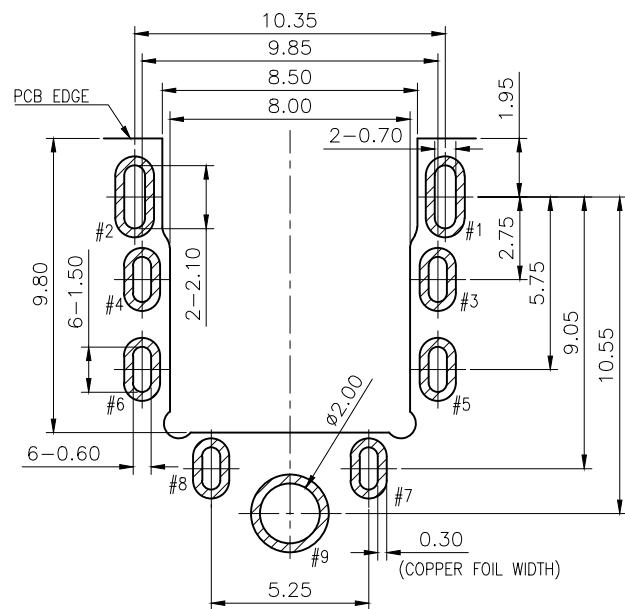
RECOMMENDED PCB LAYOUT (TOP VIEW) (TOLERANCE=±0.05mm ; THICKNESS=1.0mm)
