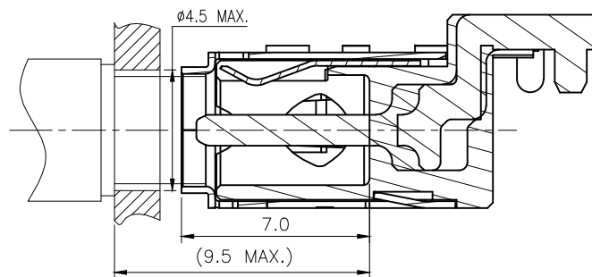
REFERENCE MATING DRAWING
